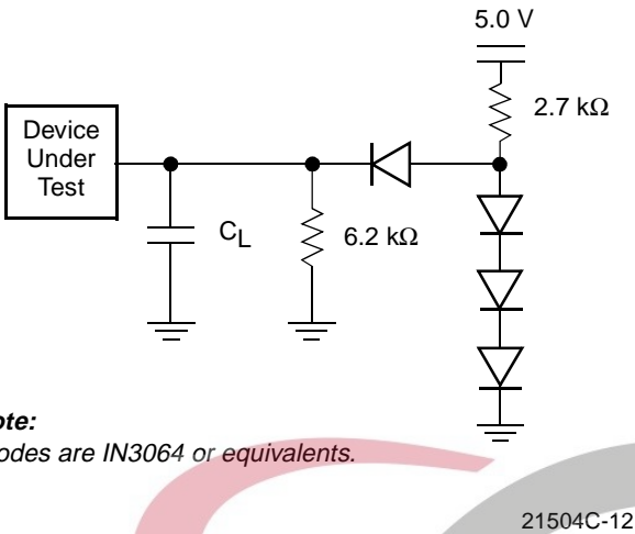
Figure 8. Test Setup
